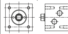
Mount Both End Cylinder "MB"
