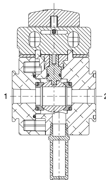
Cross Section - Series 651/652/653 Shut Off Isolation Valve
