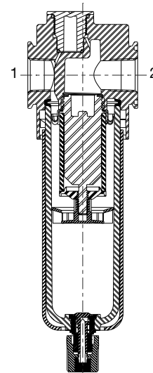
Cross Section - Series 651/652/653 Particulate Filter
