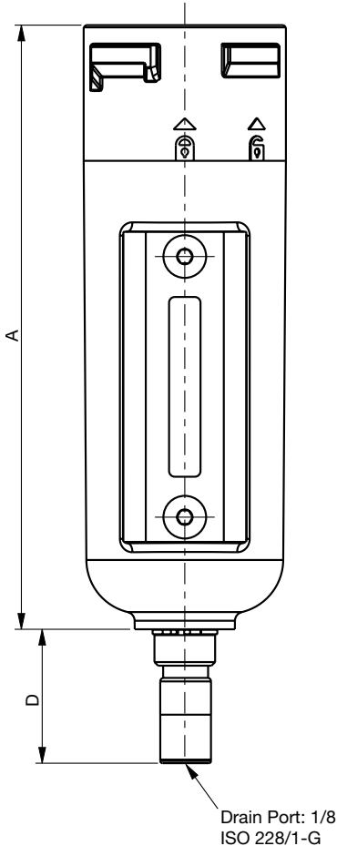
Metal Bowl with Automatic Drain
