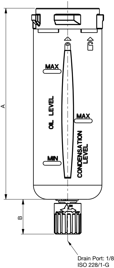
Polycarbonate Bowl/Guard with Semi-automatic/Manual Drain
