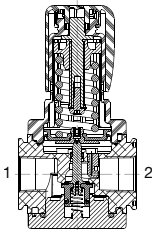
Cross Section - Series 651/652/653 Regulator
