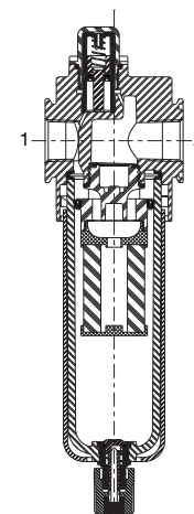
Cross Section - Series 651/652/653 Coalescing Filter
